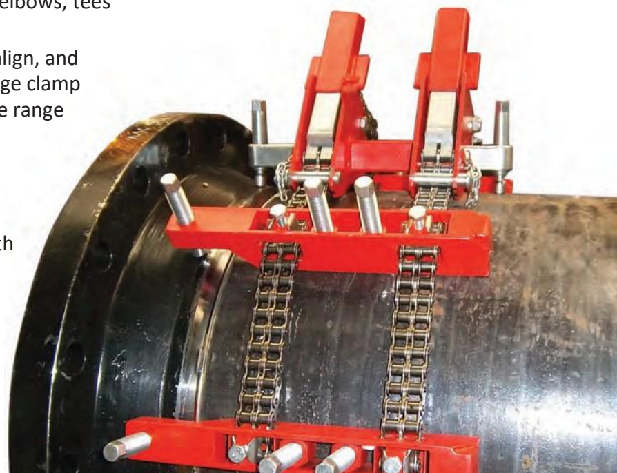
Heavy duty jackbars for arduous aligning and reforming jobs
